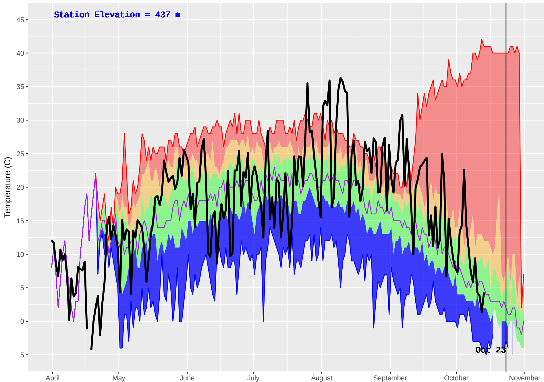
ELK MOUNTAIN (438) : Historical (1973–2016) and Current (2017) Noon Temperature
