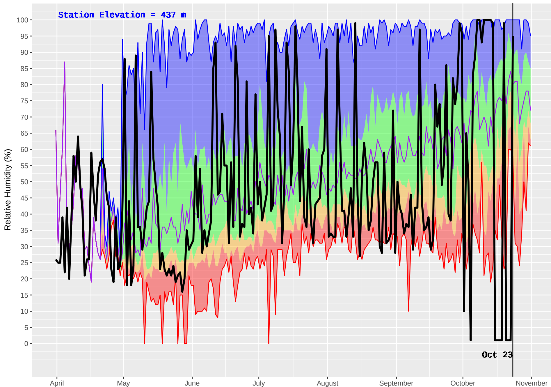
ELK MOUNTAIN (438) : Historical (1973–2016) and Current (2017) Noon Relative Humidity
